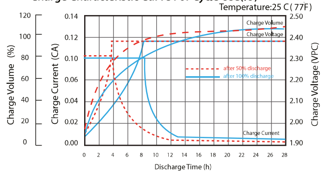
Charge Characteristic Curve For Cycle Use(IU)
